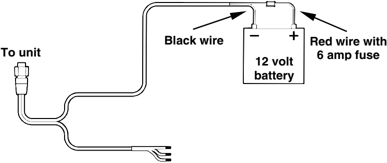
Power connections for the GlobalMap 7000C GPS unit.
